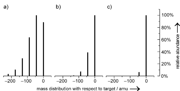
Figure 1. Statistical modeling [17] of multi-chain PEG brush: Simulated mass spectra showing the statistical distribution of 32 copies of PEG oligomers, PEG m , at specific purities attached to a single substrate. a) 96% oligomer purity [20] (taken from analysis of Quanta BioDesign amino-dPEG 24 tert -butyl ester). b) 98.8% oligomer purity (target 16-mer purity chosen as benchmark). c) 99.8% oligomer purity (taken from actual purity of amino-PEG 16 methyl ether 19 synthesized herein).
